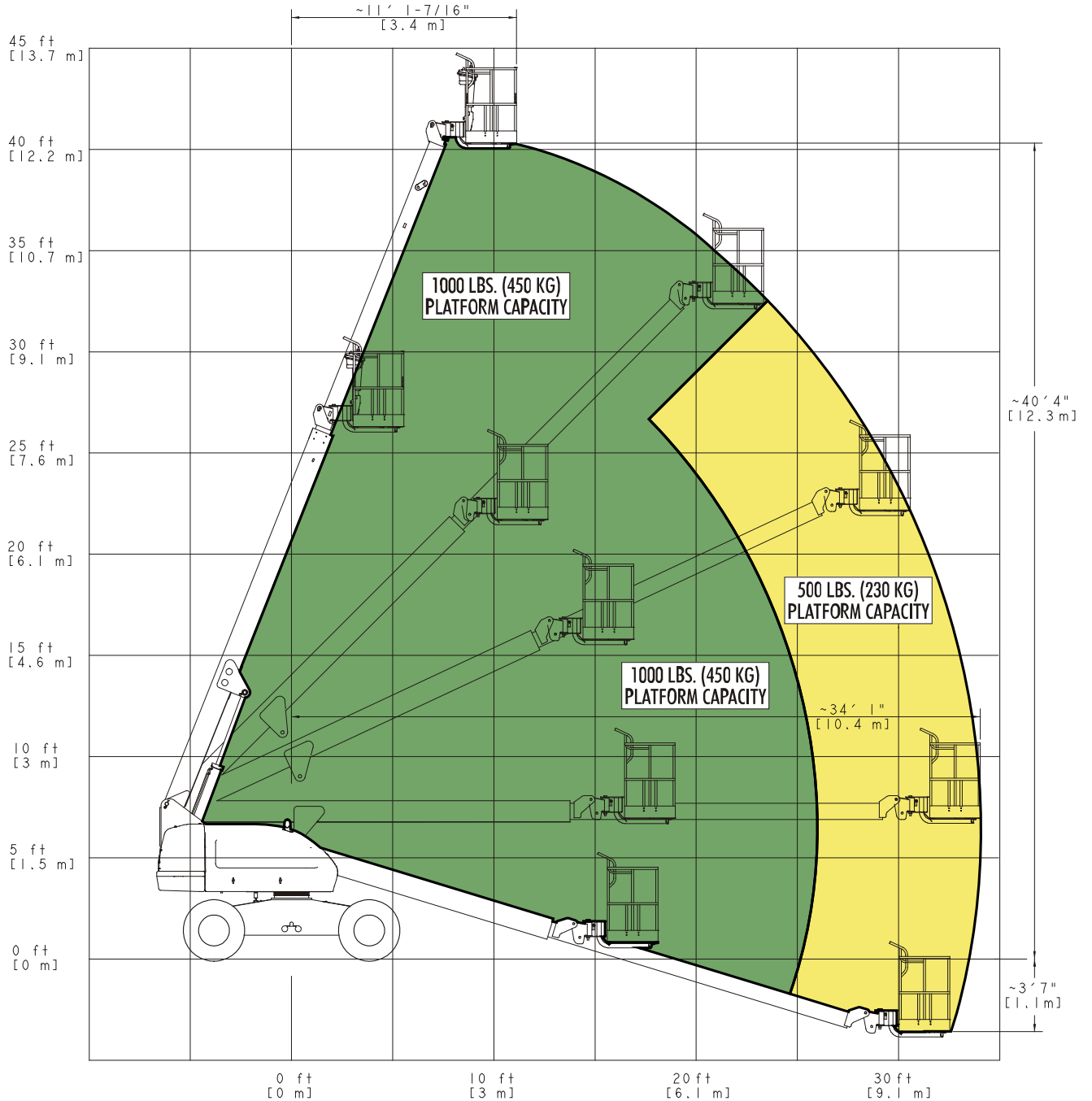
REACH DIAGRAM FOR STANDARD 500/1000 LB PLATFORM CAPACITY
